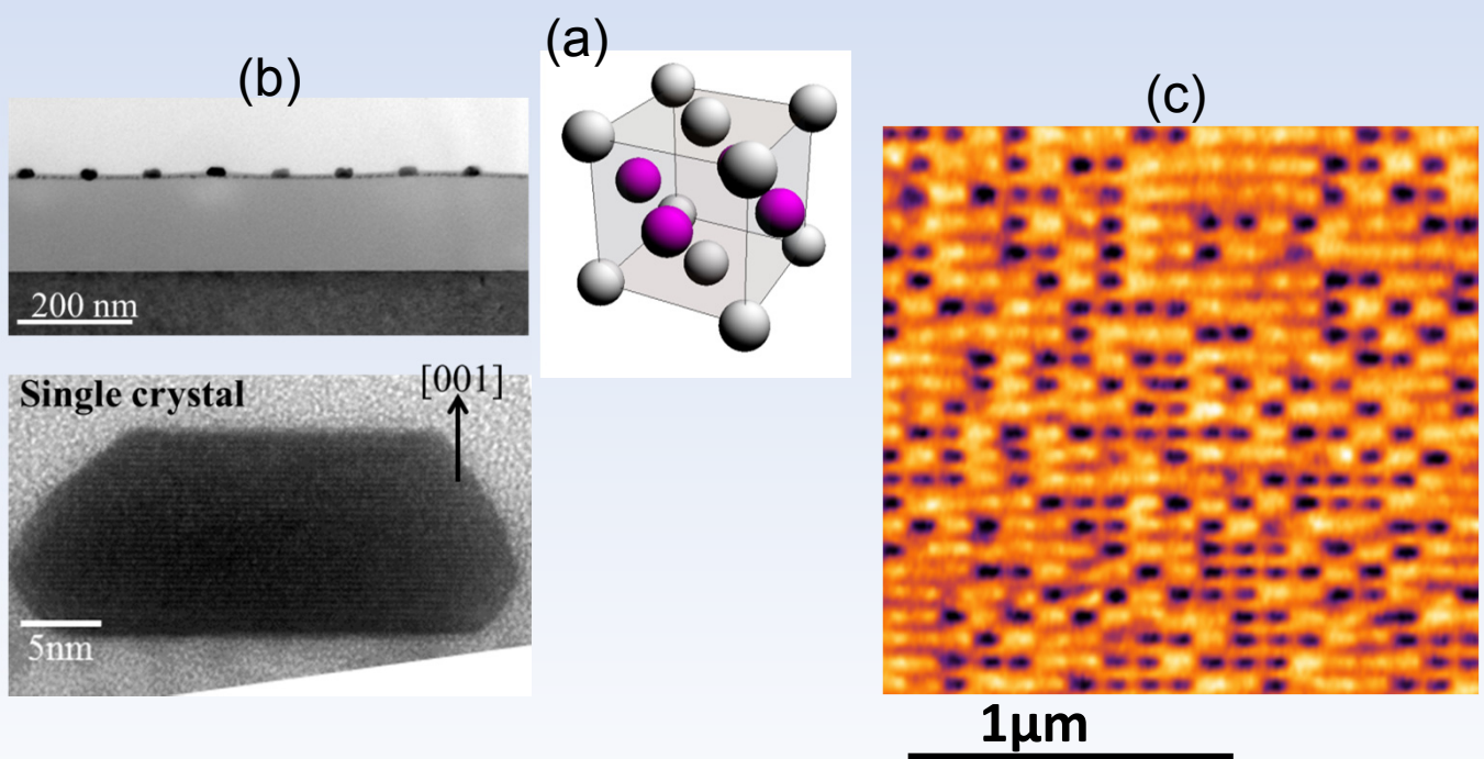
(a) L 10 FePt ordered structure, (b) cross-sectional TEM image of patterned dots, and (c) bit pattern media.
